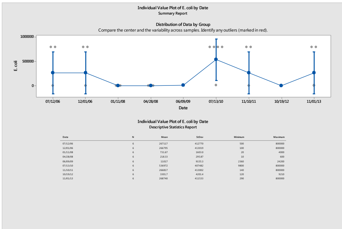
Results of annual stormwater monitoring under MS4 permit for E.coli (CFU/ 100 mL of sample) Town of Ledyard
